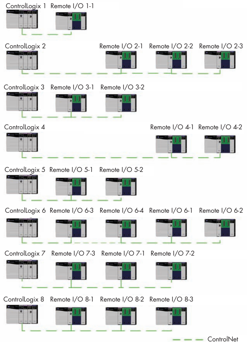
Figure 1. The control system originally planned for the food manufacturer consisted of connecting eight Allen-Bradley ControlLogix PACs to Remote I/O racks via ControlNet. The systems integrator analyzed the design and customer requirements using the Rockwell Automation Integrated Architecture Builder (IAB) software and EtherNet/IP Capacity Tool.
