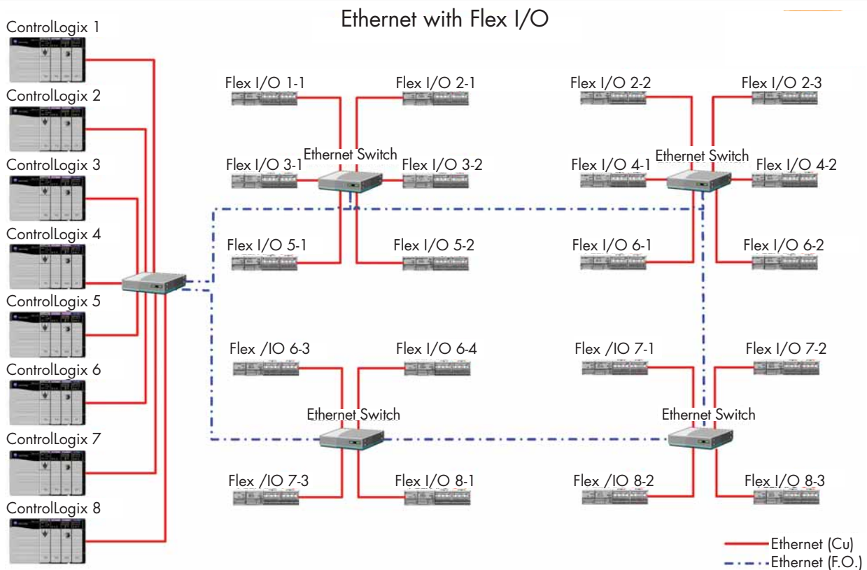
Figure 2. The project team changed the design to an Ethernet with Allen-Bradley Flex I/O. As a result, the manufacturer saved 25% on controls hardware, reduced network types in the plant and achieved smaller panel footprints.
